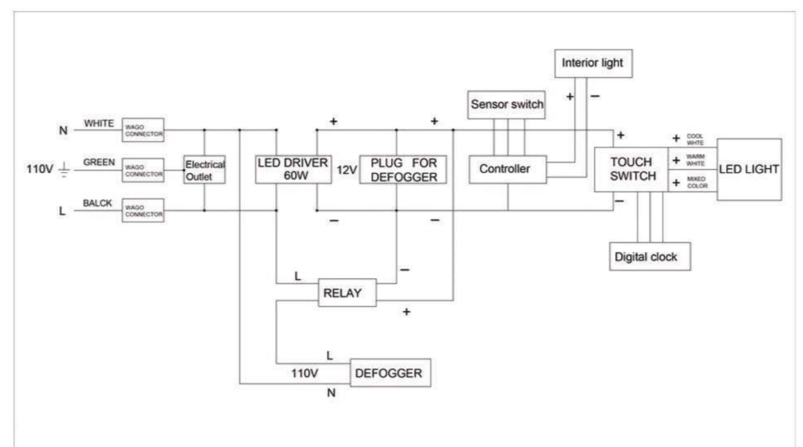
Circuit Diagram
