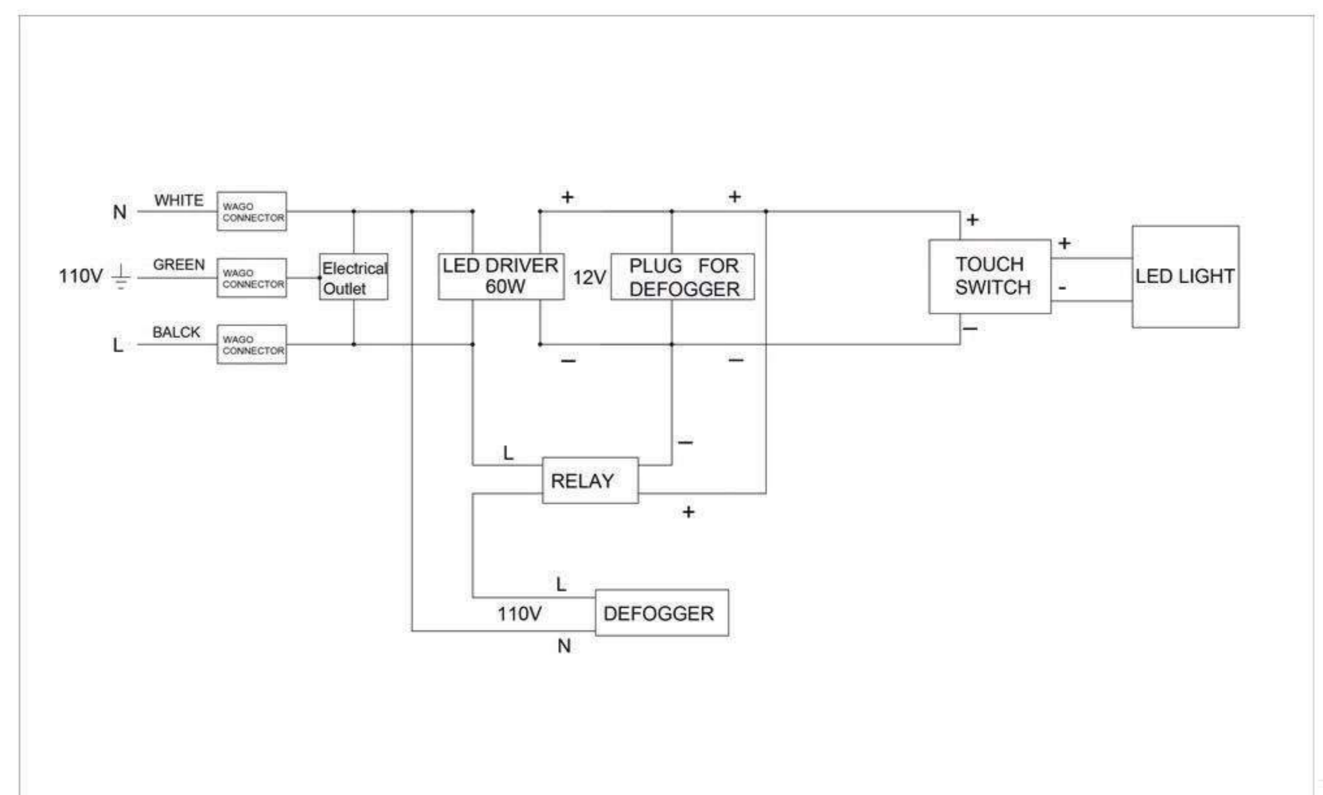
Circuit Diagram
