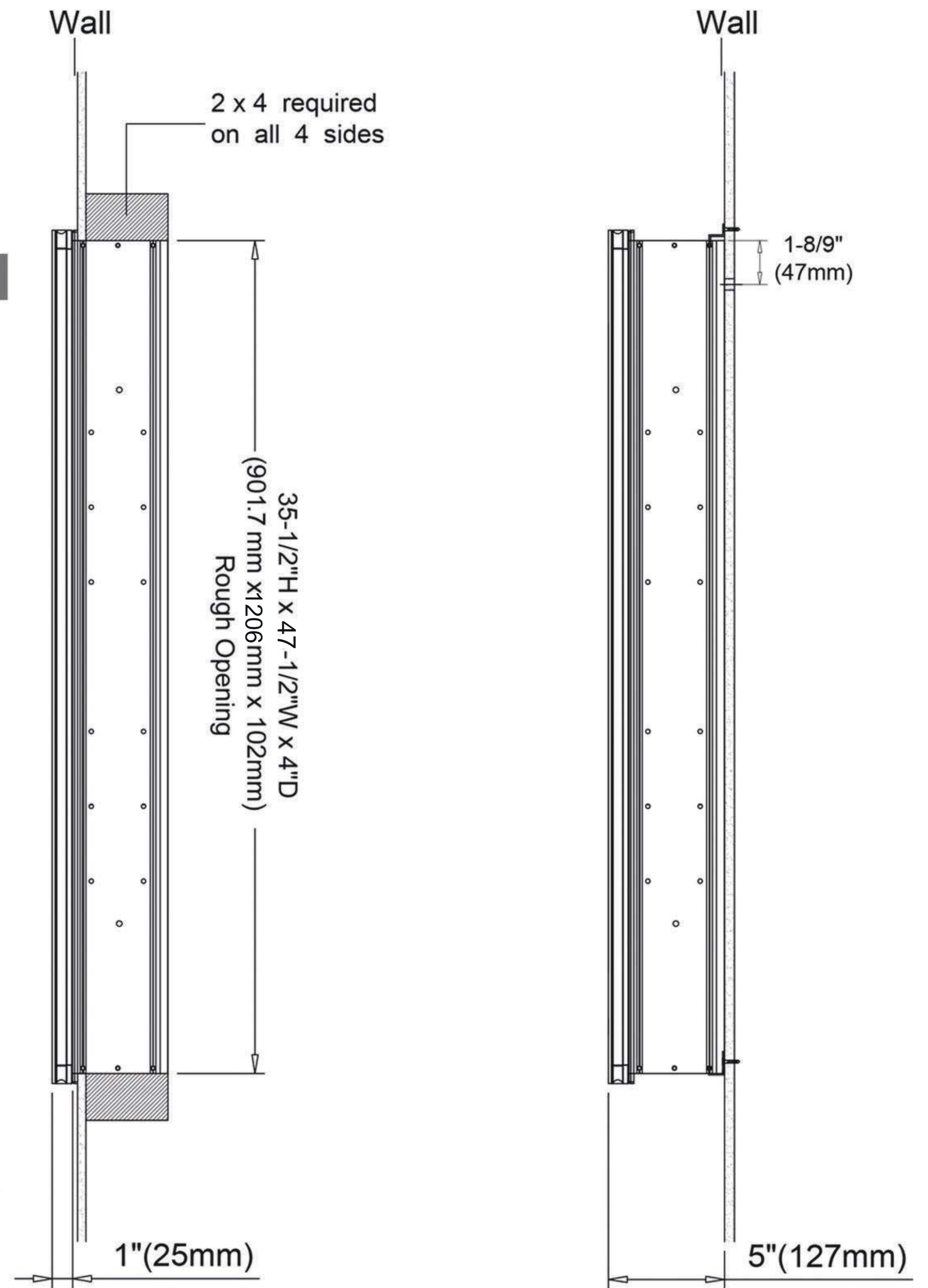
Recessed Mount
