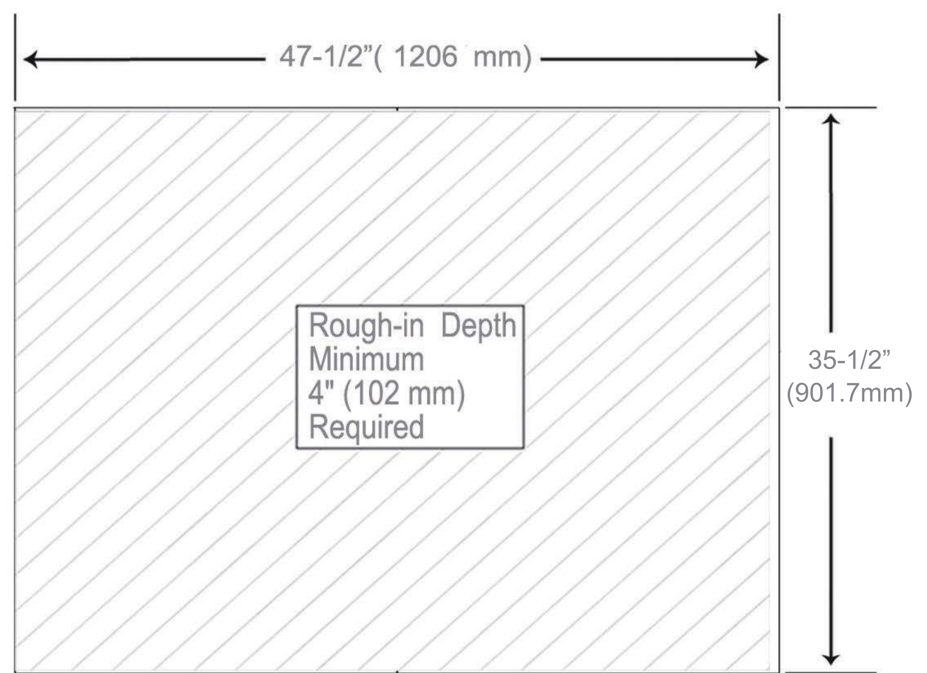
Rough-in Dimensions
