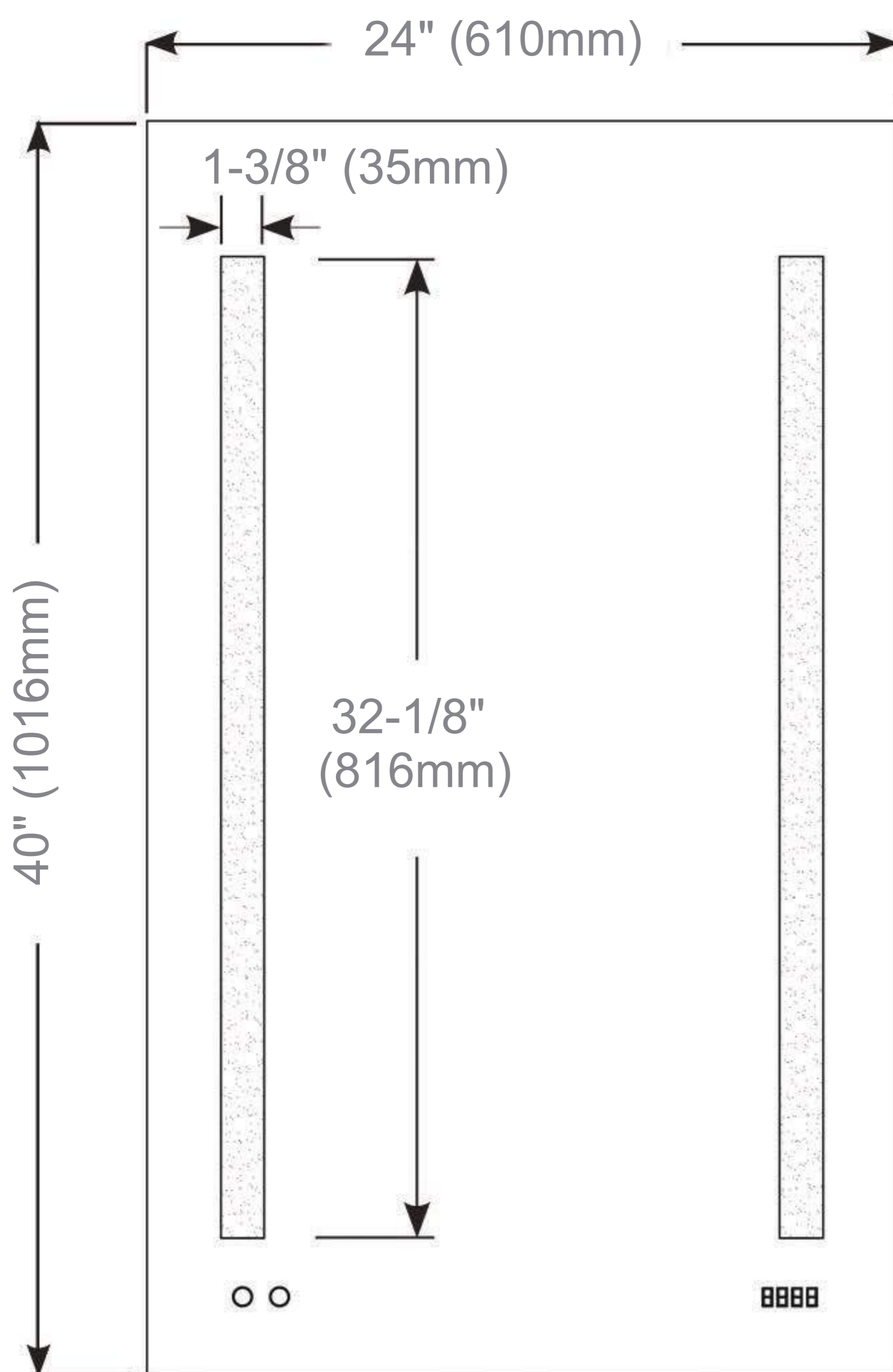
Cabinet Dimensions
