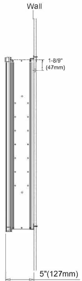
Surface Mount
