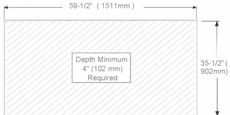
Rough-in Dimensions
