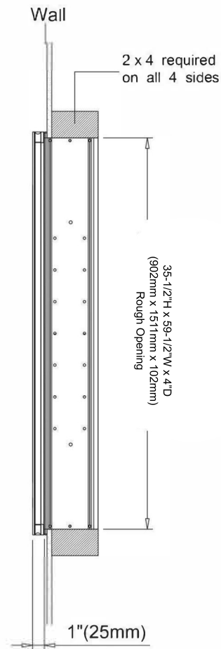
Recessed Mount
