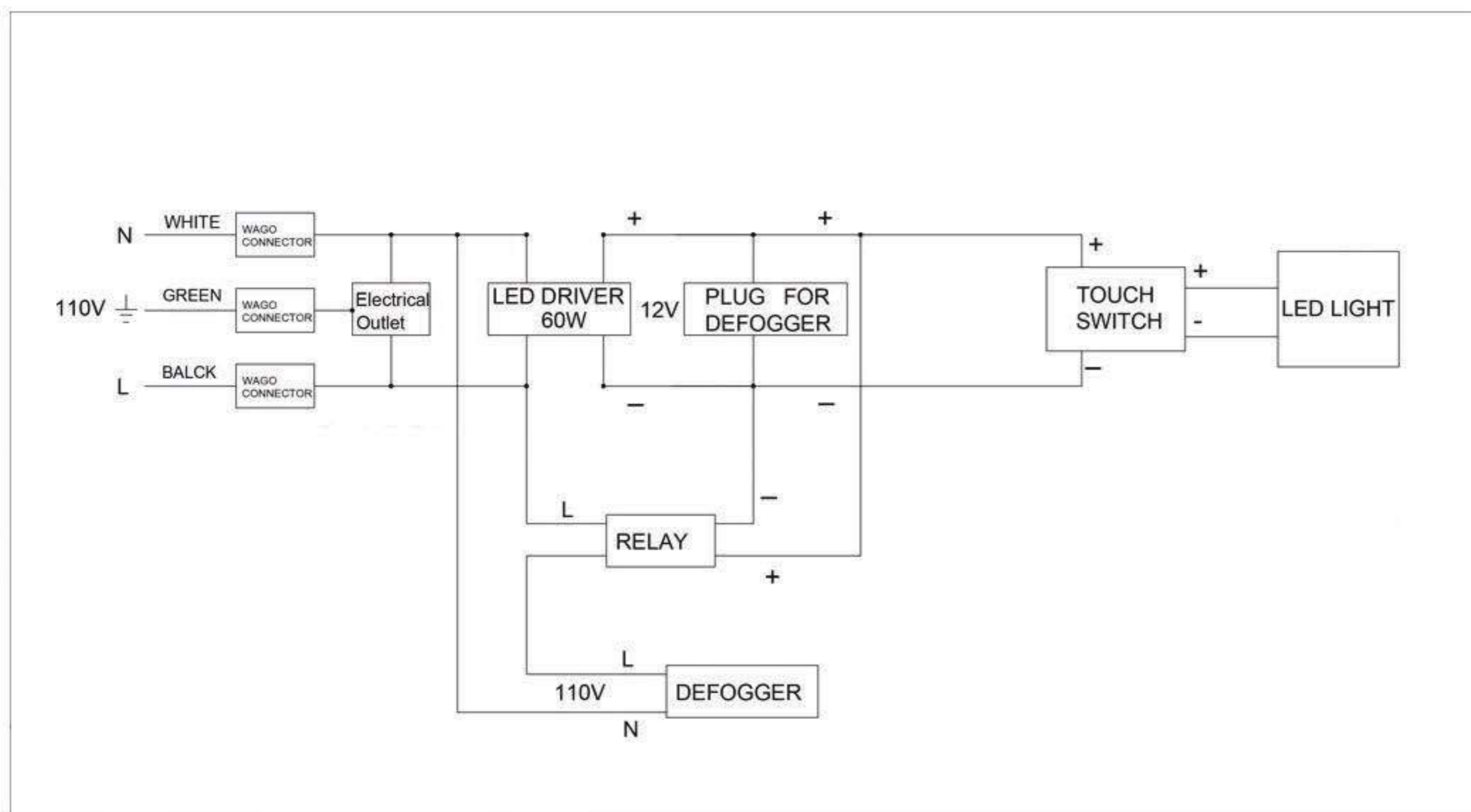
Circuit Diagram
