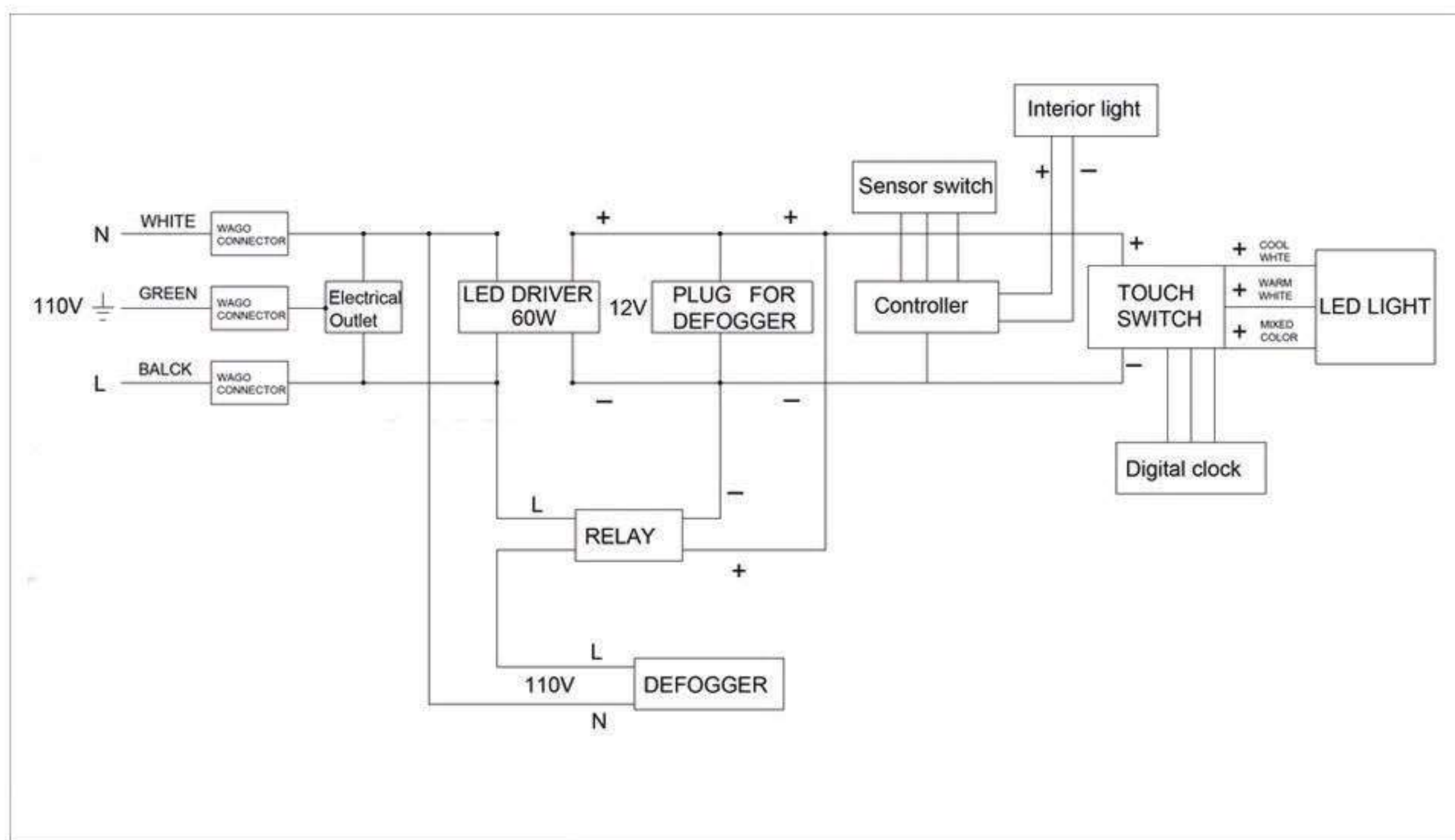
Circuit Diagram
