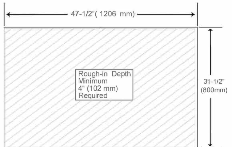
Rough-in Dimensions
