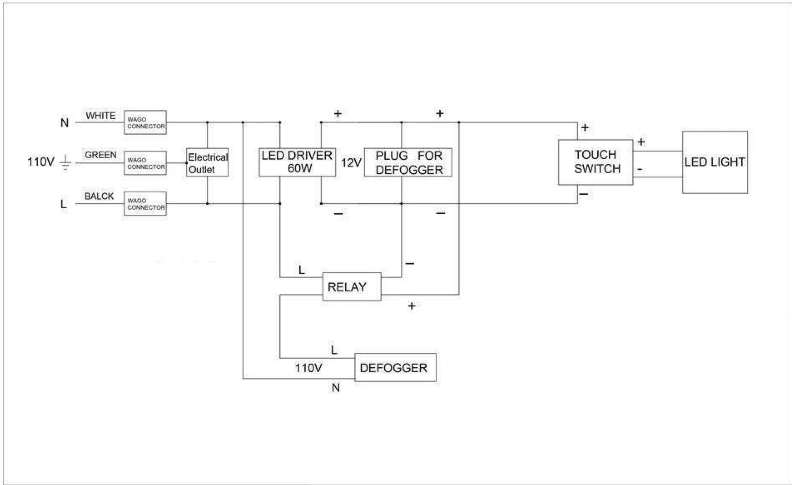
Circuit Diagram
