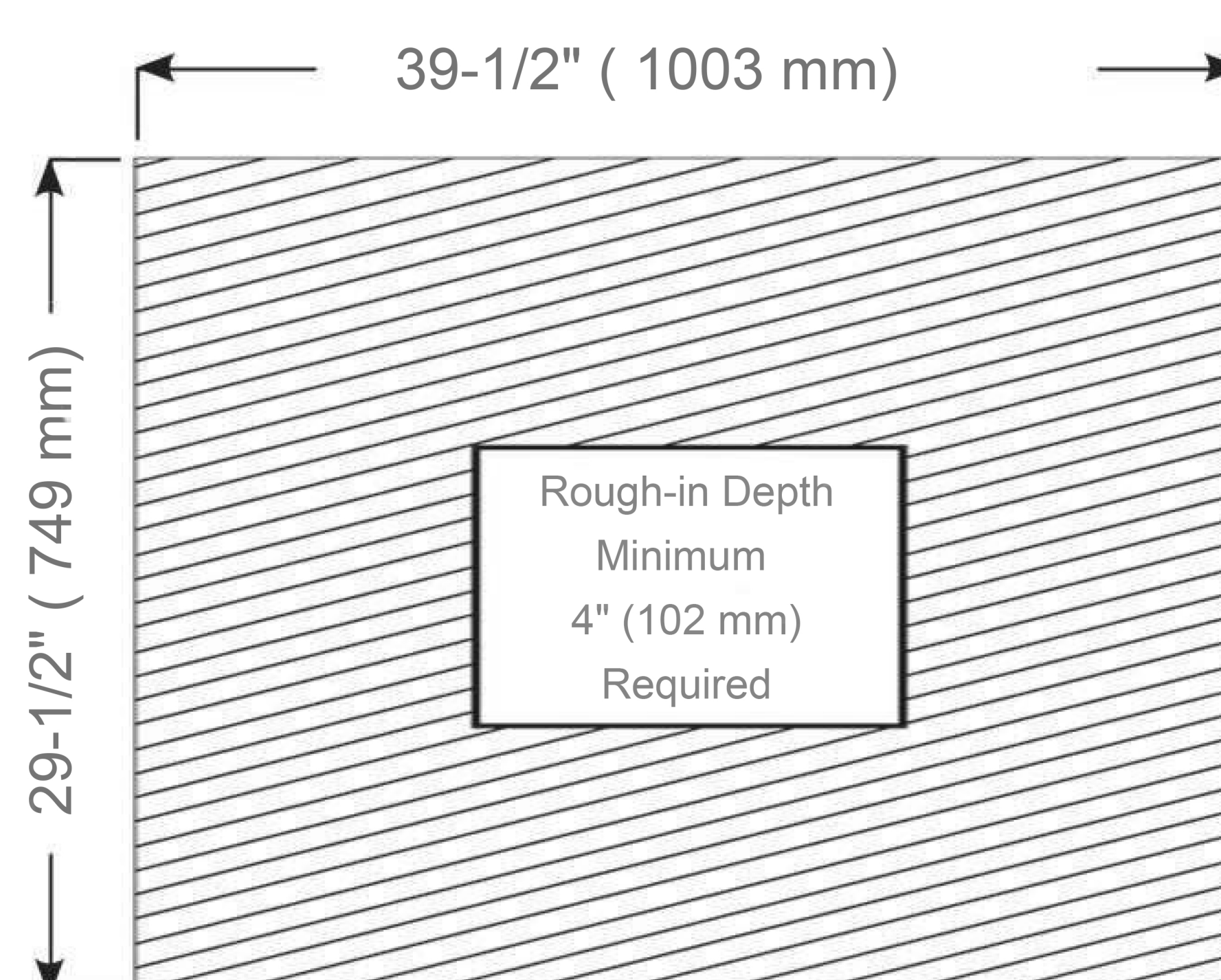
Rough-in Dimensions
