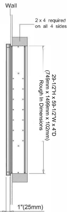
Recessed Mount
