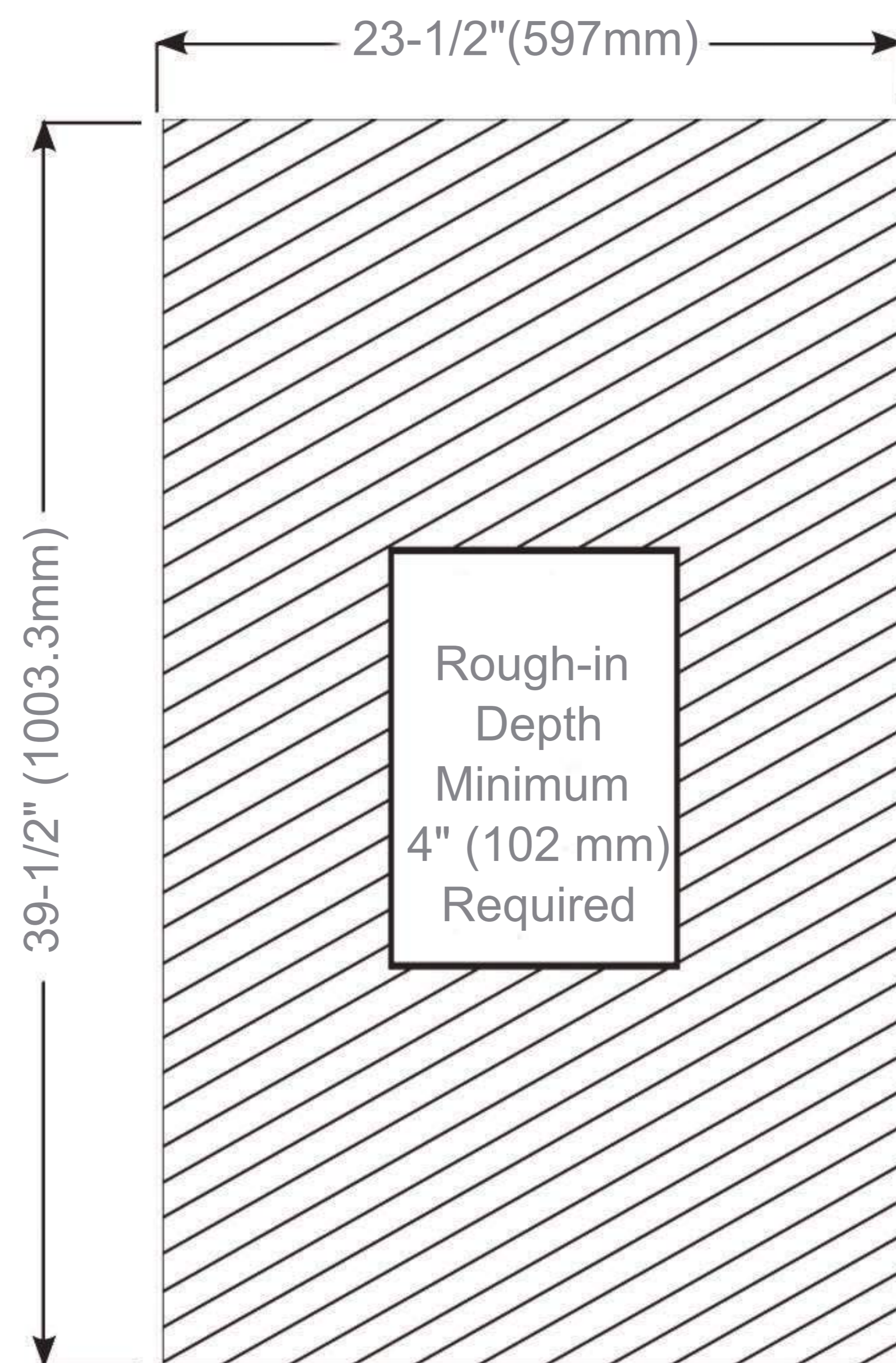
Rough-in Dimensions
